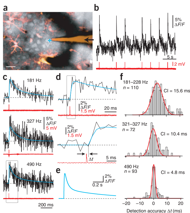
Figure 3 | Determining spike times from AOD-based optical recordings. (a) L2/3 cell population labeled with OGB-1 and sulforhodamine 101. A juxtacellular recording was obtained with a patch pipette (arrow) from the neuron marked with the five-point RAPS pattern (blue). Scale bar, 20 \mu m. (b) Simultaneous fluorescence measurement (top) and electrical recording (bottom) of one out of 51 neurons sampled at 327 Hz (neuron marked in a ). Fluorescence trace was smoothed with a five-point box filter. (c) Example 1AP-evoked calcium transients for three different cells measured for 91 neurons sampled at 181 Hz (top), 51 neurons at 327 Hz (middle) and 34 neurons at 490 Hz (bottom; dashed box indicates the close-up shown in d ). Blue traces are curve fits to the unfiltered raw fluorescence data. Dashed lines indicate zero lines. (d) Close-up of the initial phase of the calcium transient marked by the dashed box in c and the corresponding juxtacellular voltage recording (top). The onset of the fluorescence trace was fit with a rising exponential and an exponential decay (blue trace). Further zoom-in (bottom), with arrows marking the time difference, \Delta t , between the spike time predicted from the onset fit and the actual spike time (0.85 ms in this case). (e) Average 1AP-evoked calcium transient pooled over all confirmed 1AP events independent of cell sampling rate ( n = 250 ). (f) Summary histograms of the distribution of \Delta t measured under the three sampling conditions. CI, 95% confidence intervals obtained from Gaussian fits (red curves; n is total number of events in each group).
